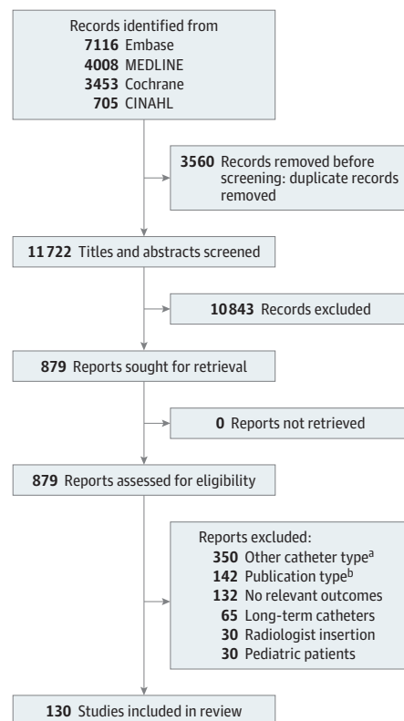
Figure 1. PRISMA Diagram
